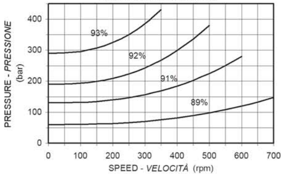
MECHANICAL EFFICIENCY RENDIMENTO MECCANICO
